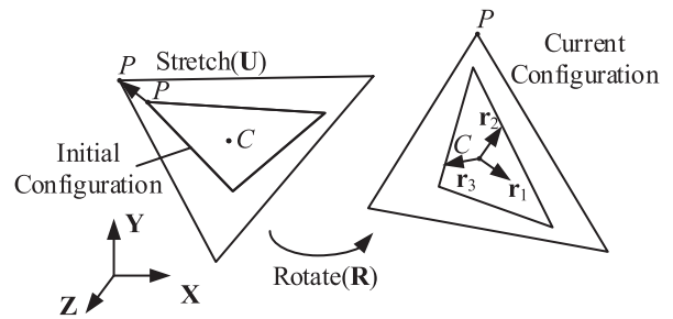
Figure 2 Polar decomposition.
