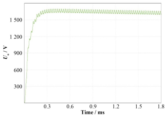
图8 逆变电源仿真输出 Fig.8 Simulation output of inverter power supply
