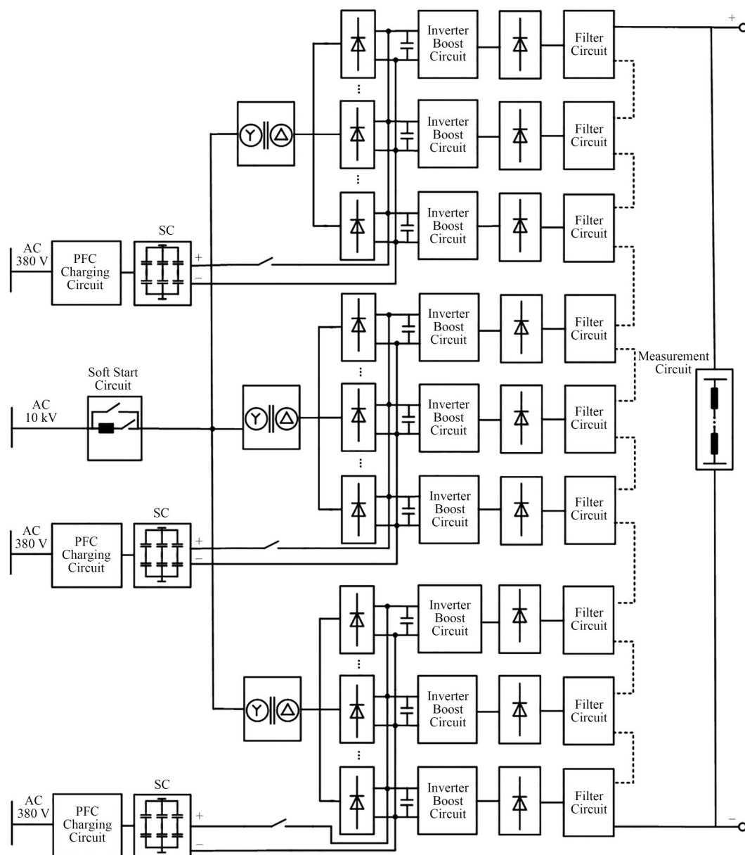
图1 逆变电源系统结构拓扑 Fig.1 Topology diagram of inverter power system structure
