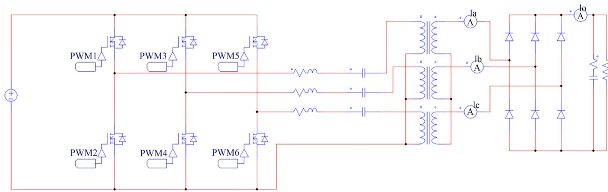
图5 LLC电路PSIM仿真模型 Fig.5 PSIM simulation model for LLC circuit
