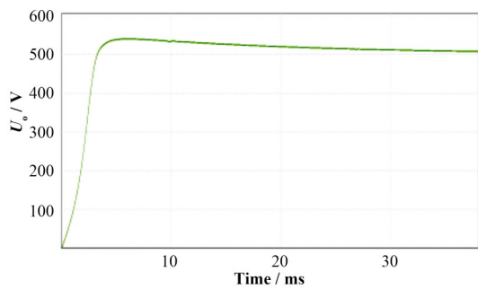
图6 LLC电路仿真输出 Fig.6 Simulation output of LLC circuit
