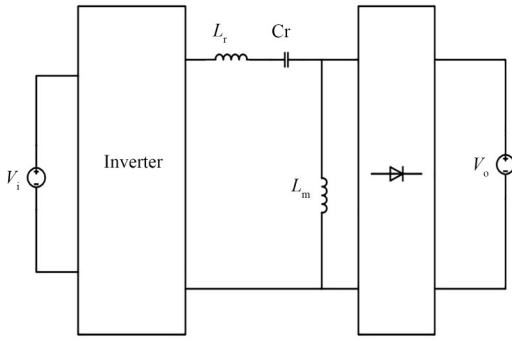
图 4 LLC 等效电路图 Fig.4 LLC equivalent circuit diagram
