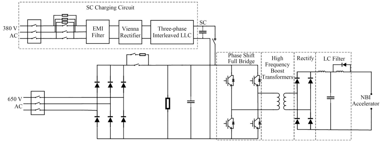
图2 逆变电源主回路拓扑 Fig.2 Topology diagram of inverter power supply main circuit
