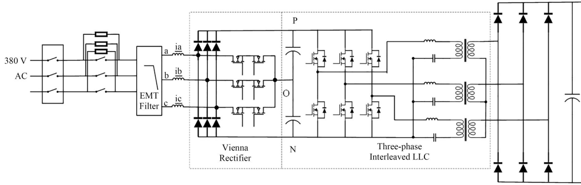
图2 逆变电源主回路拓扑 Fig.2 Topology diagram of inverter power supply main circuit
