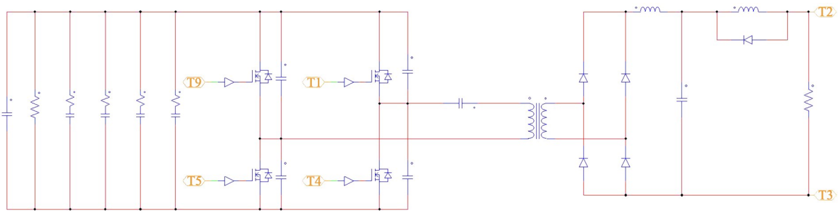
图7 逆变电源PSIM仿真模型 Fig.7 PSIM simulation model for inverter power supplies
