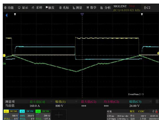
图11 软开关性能测试(彩图见网络版) Fig.11 Performance testing of soft switch (color online)
