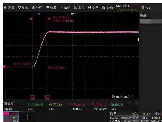
图9 阶跃响应性能测试 Fig.9 Performance testing of step response
