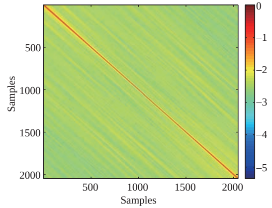
Figure 5 Coherence matrix of \mathbf{A} .
