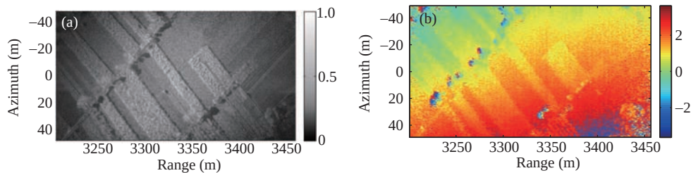
Figure 11 Chirp scaling results. (a) Magnitude; (b) interferometric phase.
