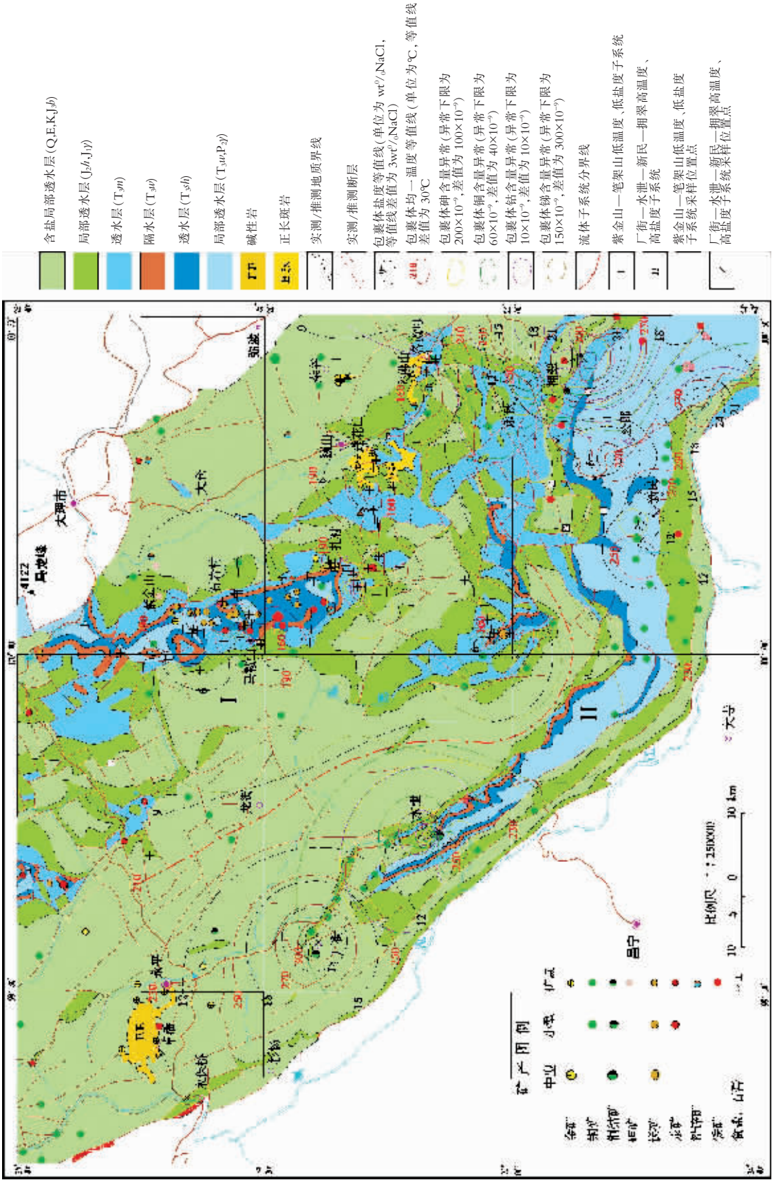
图 1 云南巍山—永平地区流体地质图 Fig. 1 Fluid-geological map of the Weishan-Yongping district, Yunnan
